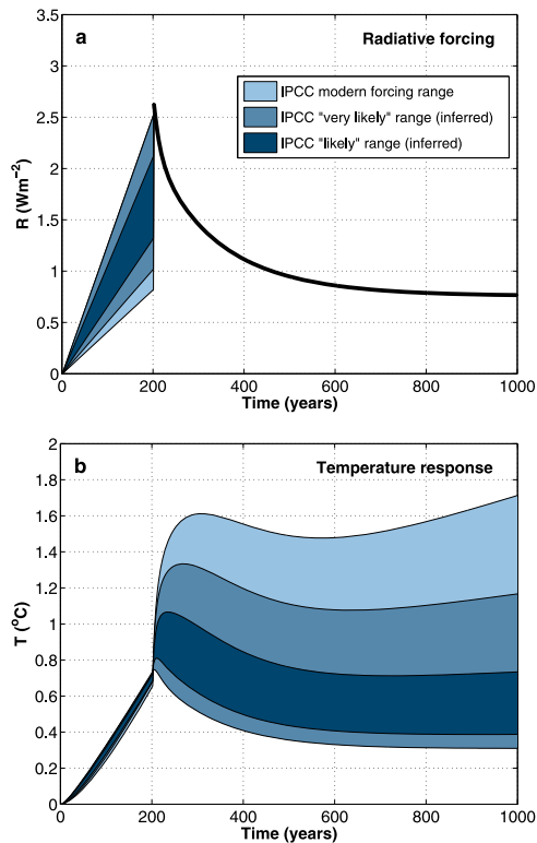
Figure 2. Illustration of what IPCC bounds on climate sensitivity imply for constraints on past climate forcing and future temperature response. (a) Radiative forcing and (b) temperature response, as in Figure 1. The dark blue shading shows the IPCC AR4 ‘likely’ range of climate sensitivity ( 2^{\circ}\text{C} to 4.5^{\circ}\text{C} ). The medium blue shading shows the IPCC AR4 ‘very likely’ range of climate sensitivity ( 1.5^{\circ}\text{C} to 10^{\circ}\text{C} —IPCC AR4 [Hegerl et al., 2007] truncates the probability distributions of climate sensitivity at 10^{\circ}\text{C} so we take this value as representative of the upper bound on the ‘very likely’ range). For comparison, the light blue shading shows the 90% confidence interval as allowed by observations, as in Figure 1. A wedge in the lower range of possible forcing translates to a wedge in the higher range of possible temperature response.
