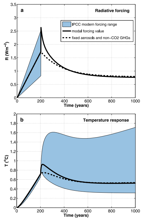
Figure 1. Observational constraints on climate forcing and temperature response. (a) Idealized representation of forcing trends. Forcing is ramped linearly to its modern value in year 200, and a zero emissions scenario is assumed thereafter. Upon zero emissions, aerosols and tropospheric ozone are specified to fall to pre-industrial levels immediately. Long-lived greenhouse gases decline at their respective ( e -folding) time scales [Forster et al. , 2007]: 12 years for methane; 114 years for nitrous oxide; 75 years (a representative lifetime) for halocarbons. Carbon dioxide falls to 40% of its peak value (above pre-industrial) with a decay time scale of 170 years [Forster et al. , 2007]. Radiative forcing is calculated using the simplified expressions of Myhre et al. [1998]. The light blue shading is the 90% confidence interval on trajectories of R as allowed by observations, where only uncertainty in aerosols is considered. The solid black line shows the modal value of R . The dashed black line shows a scenario in which aerosols and non- \text{CO}_2 greenhouse gases are held fixed at their modern concentrations upon the elimination of \text{CO}_2 emissions. (b) As for Figure 1a, but modeled temperature response. Values of \lambda have been paired with values of R so that individual temperature trajectories are tightly constrained, analogous to the situation for modern observations.
